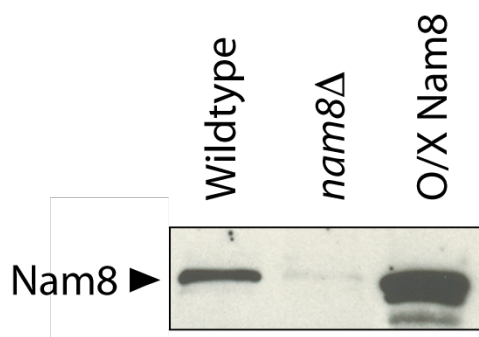
Figure 2. Abundance of Nam8 protein in various strains of Saccharomyces cerevisiae as determined by Western blot. S. cerevisiae extract (50 \mu g total protein) was separated by 10% SDS-PAGE and blots were probed with \alpha -Nam8 antibodies. Extracts shown are from wildtype S. cerevisiae , a strain lacking the NAM8 gene ( nam8Δ ), and a strain that overexpresses the NAM8 gene (O/X Nam8). The position of the Nam8 protein is indicated by an arrowhead.
